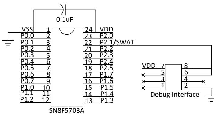
example circuit
