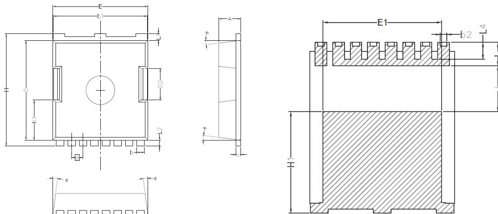
TOLL-8L Package
