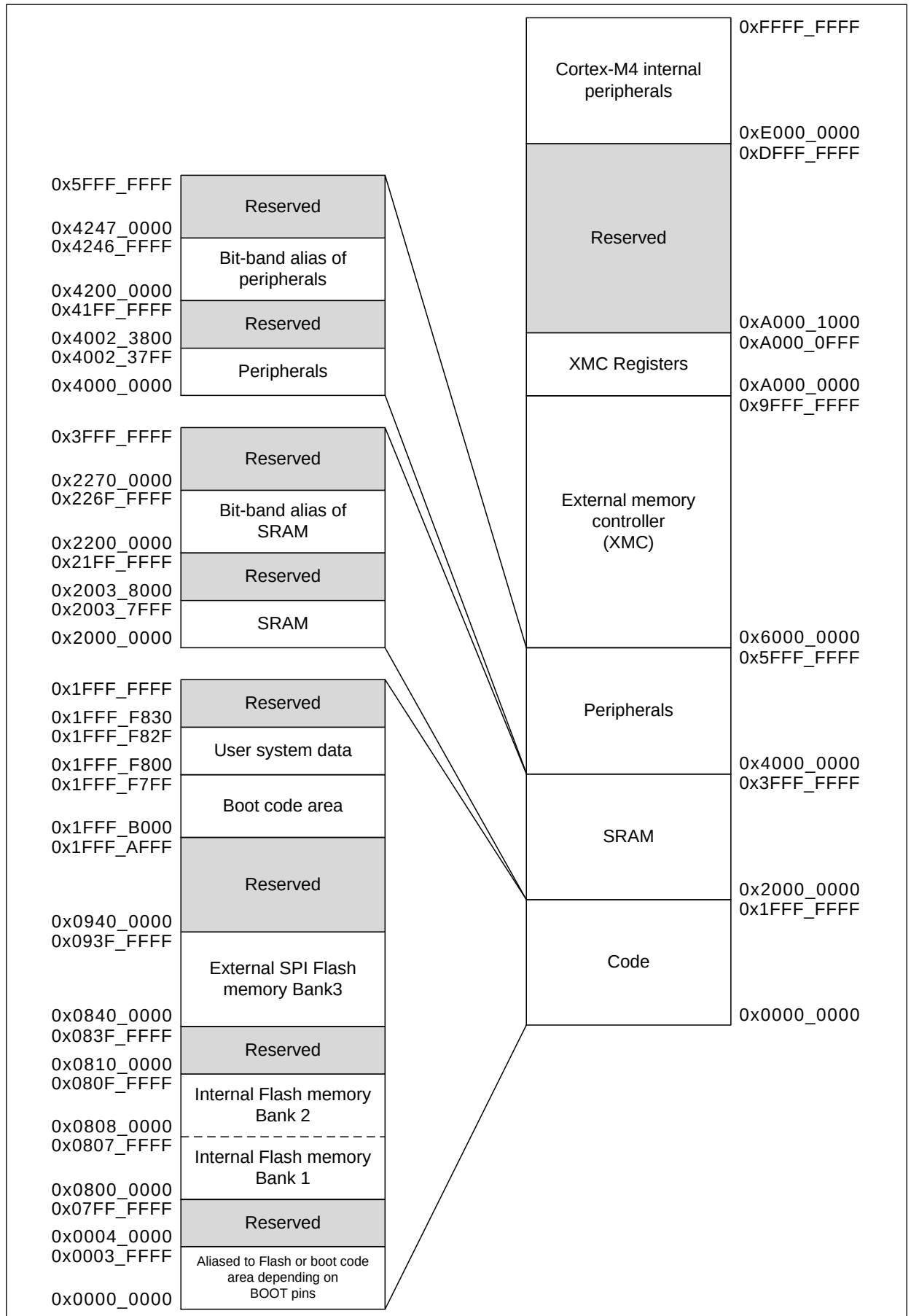
Figure 4. Memory map
