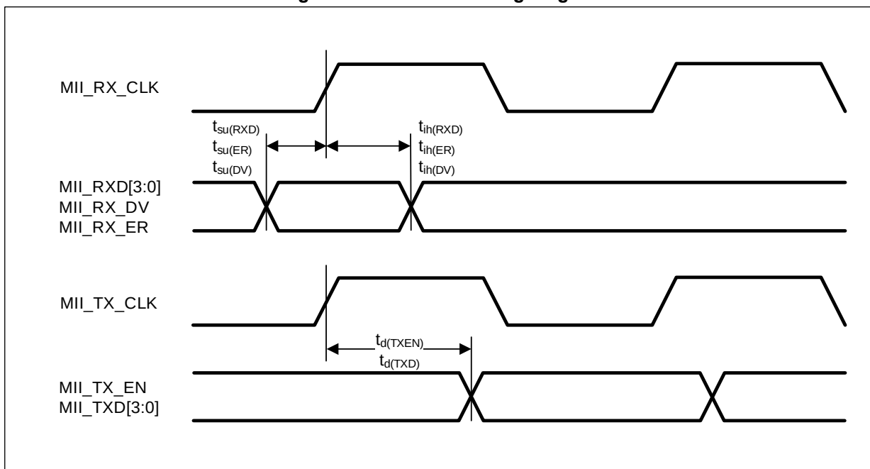
Figure 34. EMAC MII timing diagram
