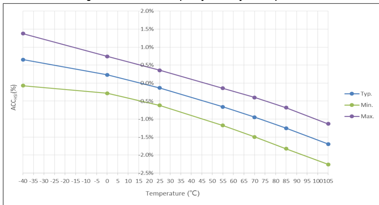
Figure 14. HICK clock frequency accuracy vs. temperature
