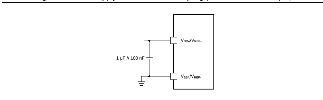
Figure 38. Power supply and reference decoupling (without external V REF pin)
