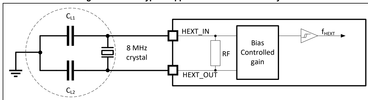
Figure 10. HEXT typical application with an 8 MHz crystal
