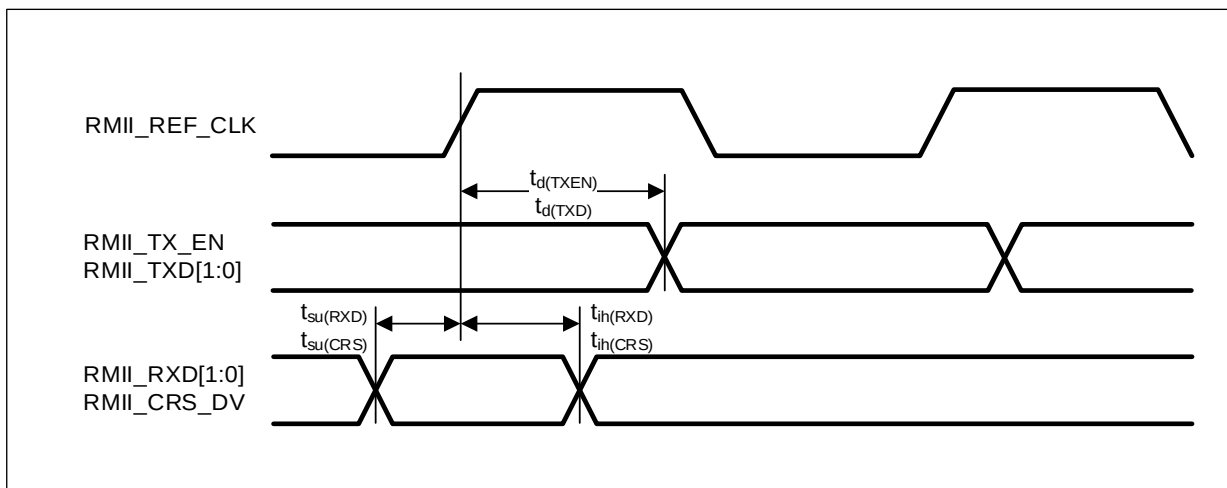
Figure 33. EMAC RMII timing diagram
