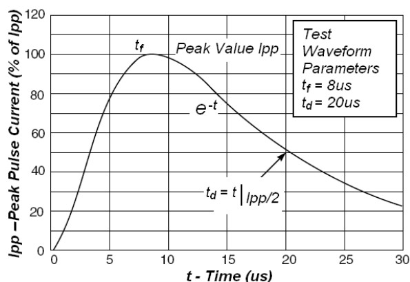
Fig1. Pulse Waveform
