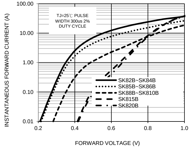
FIG. 2-TYPICAL FORWARD CHARACTERISTICS
