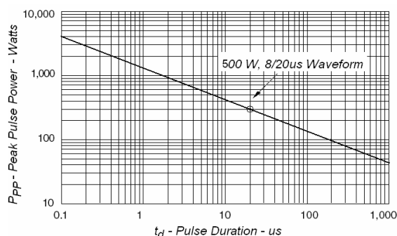
Fig1. Peak Pulse Power VS Pulse Time
